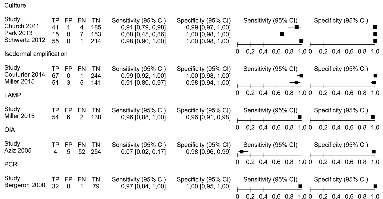
Fig. 4. Forest plot of comparator/reference test for GBS detection. Abbreviations: CI, confidence interval; FN, false negative; FP, false positive; LAMP, loop-mediated isodermal DNA amplification; OIA, optical immunoassay; PCR, polymerase chain reaction; TN, true negative; TP, true positive.
